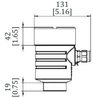
Single Chamber Housing
