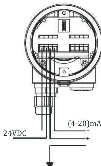
24V DC Four-wire
