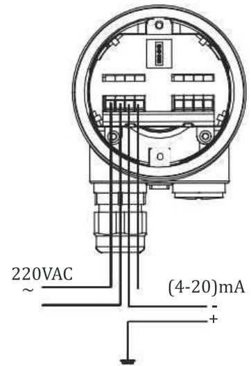
220V AC Four-wire
