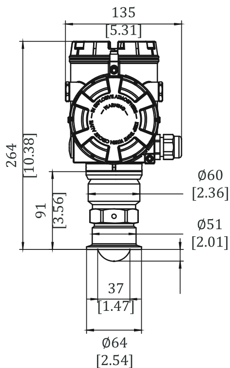
RLT6400S with Hygienic Connection
