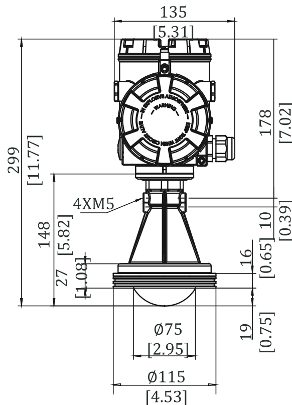
RLT6400P with Plastic Horn Antenna
