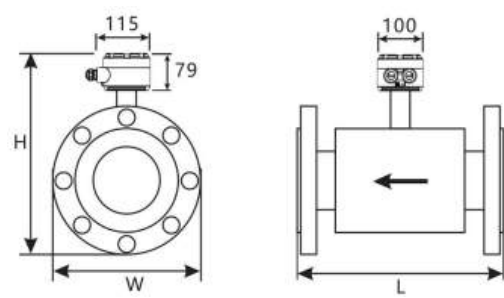
Flange (separate type)
