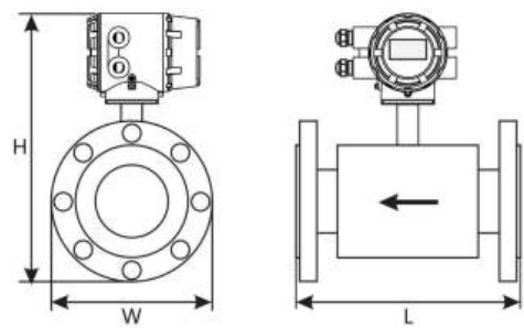
Flange type (integrated type)
