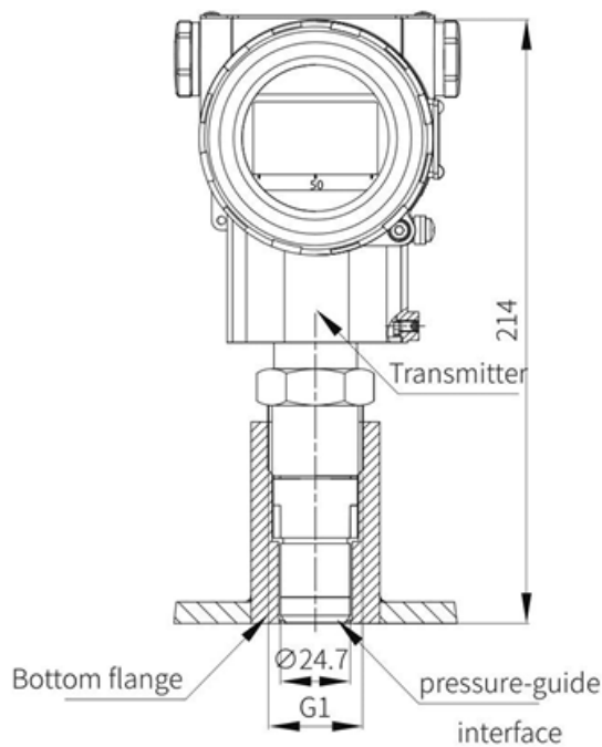
G1 thread connection Pulp joint (code L)
