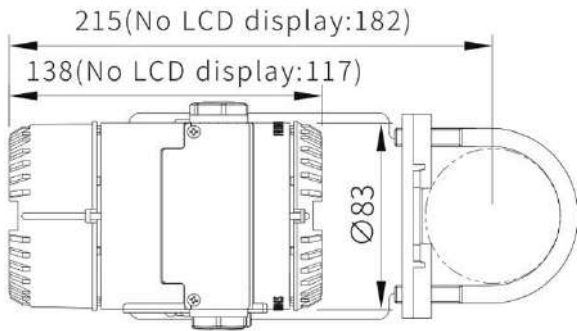
Horizontal Piping Connection Type (Side)
