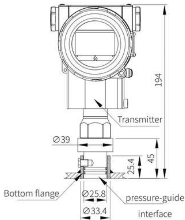
φ25.8 inserted connection Pulp joint (code S)
