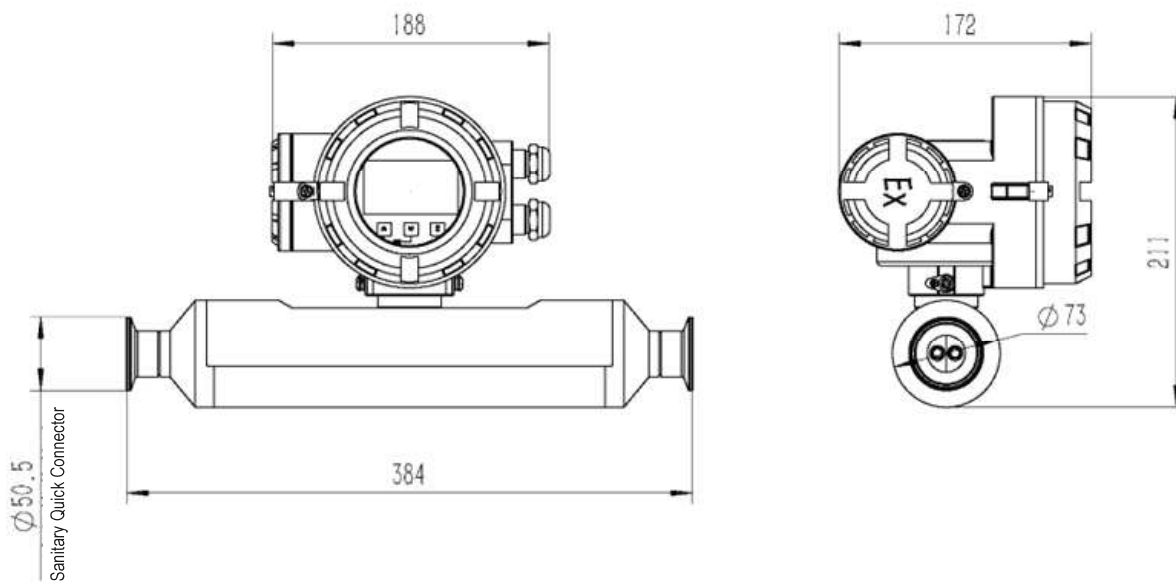
Ascending pipe structure sensor (Integrated mounting type)
