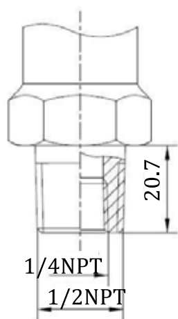
1/2" NPT Male Thread (Code 2)
