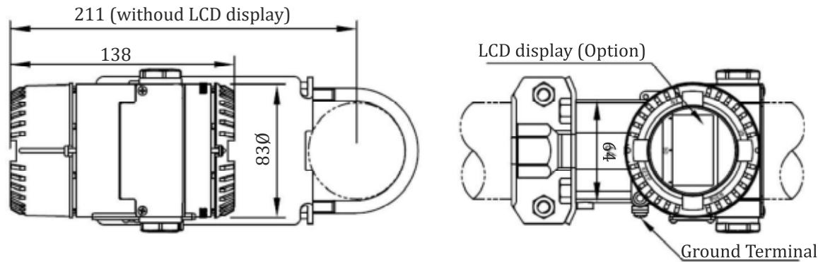
Horizontal Piping Connection Type (Side)
