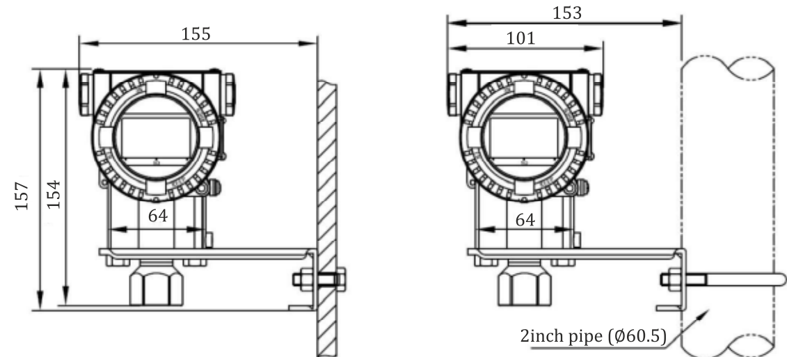
Wall Mounting Connection Type
