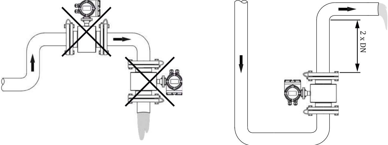
Installation in pipe without emptying
